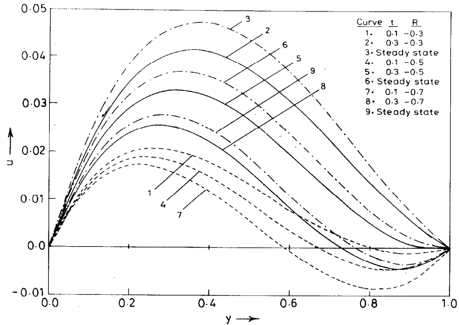
Fig.2. Velocity profiles of air ( Pr = 0.71 ) when R < 0 .
